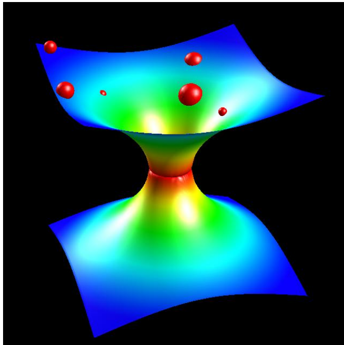
FIG. 3: An artist’s representation of the extended space-time of loop quantum cosmology. Time again runs vertically. General relativity provides only the top half of this space-time which originates in the Big Bang (see figure 2). Quantum Einstein’s equations extend this space-time to the past of the Big Bang. The pre-Big Bang branch is contracting and the current post-Big Bang branch is expanding. The band in the middle represents the ‘quantum bridge’ which joins the two branches and provides a deterministic evolution across the ‘deep Planck regime’. Image: courtesy of Dr. Cliff Pickover, www.pickover.com
