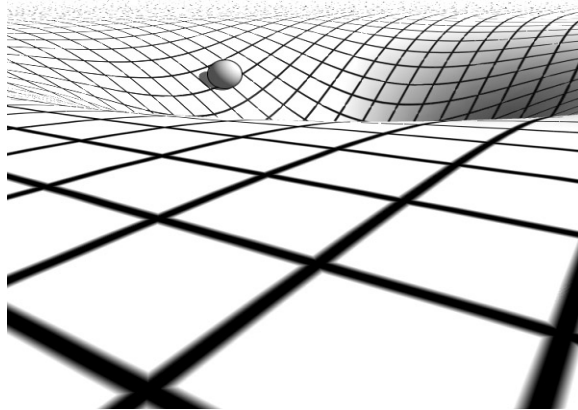
FIG. 1: An artist's depiction of planetary motion in general relativity. Heavy bodies such as our sun bend space-time. Planets go 'as straight as they can' in this curved geometry. In the flat space perspective of Newtonian physics, however, the same orbits appear to be elliptical, being eternally pulled to the sun by gravity. Thus the familiar gravitational force of Newtonian physics is just a 'poor man's way' of describing effects of space-time curvature using a flat space framework. Image: Boris Starosta, www.Starosta.com
